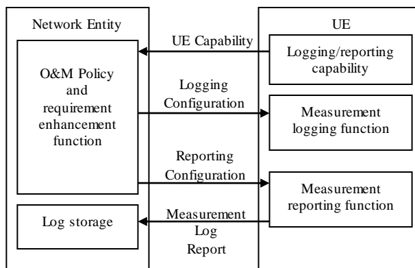
Fig. 2. UE Feedback scheme
