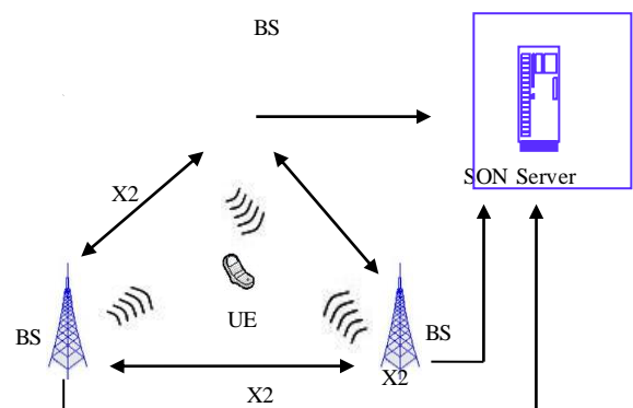
Fig. 1. Network Analytics by UE assisted measurements in E-UTRAN
